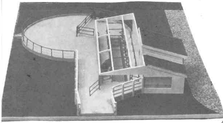
MODEL OF A HERRINGBONE MILKING SHED MADE BY R. PLAISTOWE
